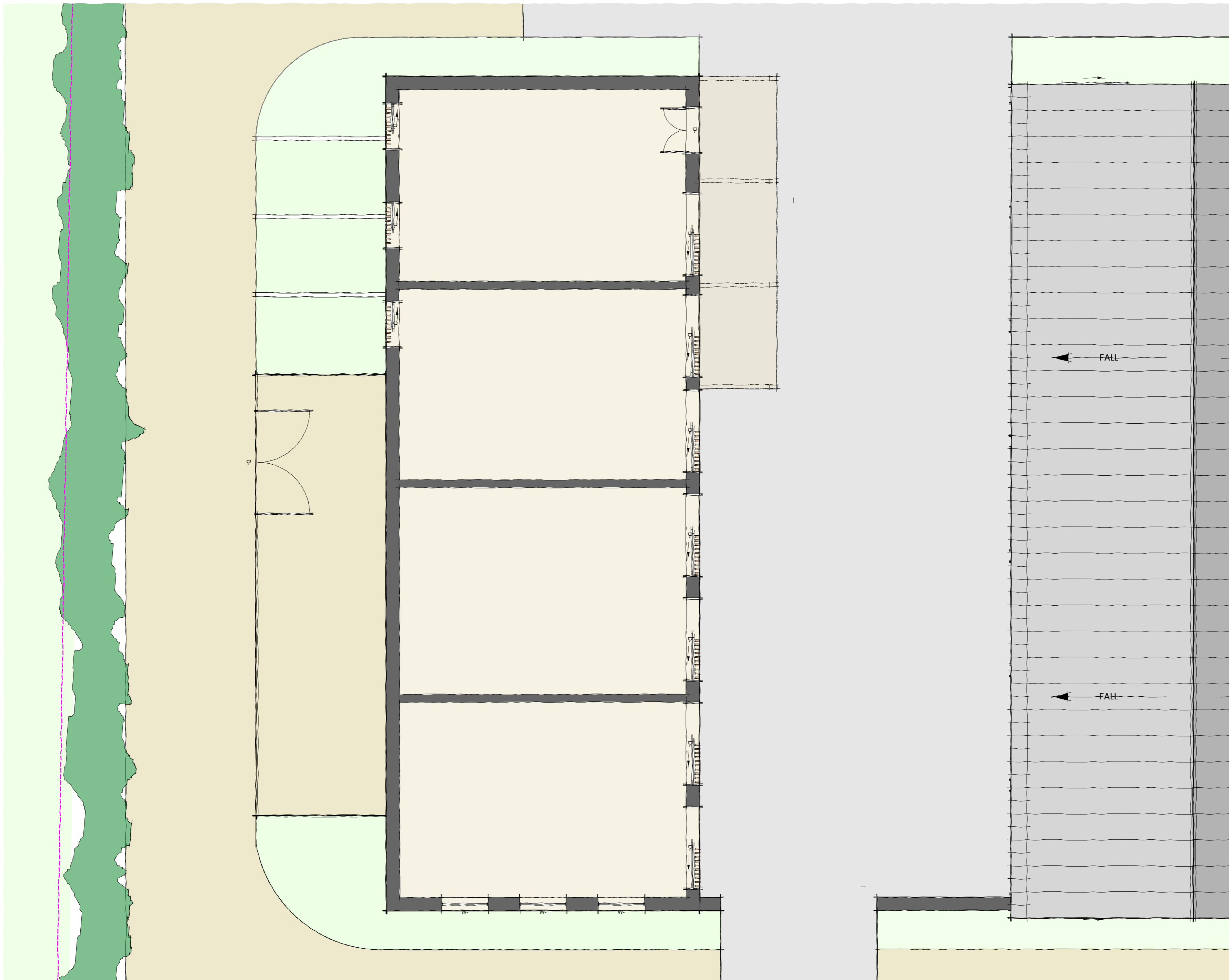
Proposed Floor Plan - Barn 2 Scale: 1:100 @ A2
