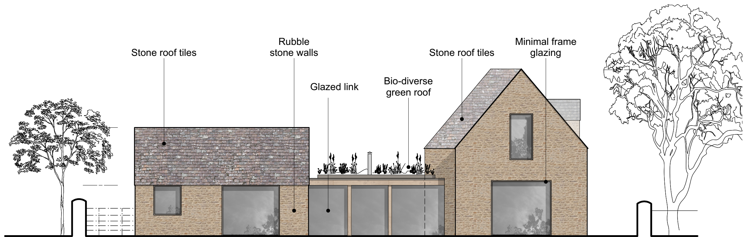
1 Bedroom 1, 2 & 3 South Elevation Scale: 1:100
