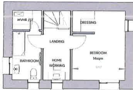
FIRST FLOORPLAN
